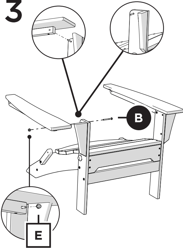
2.5" Screw — H.27X2.5
